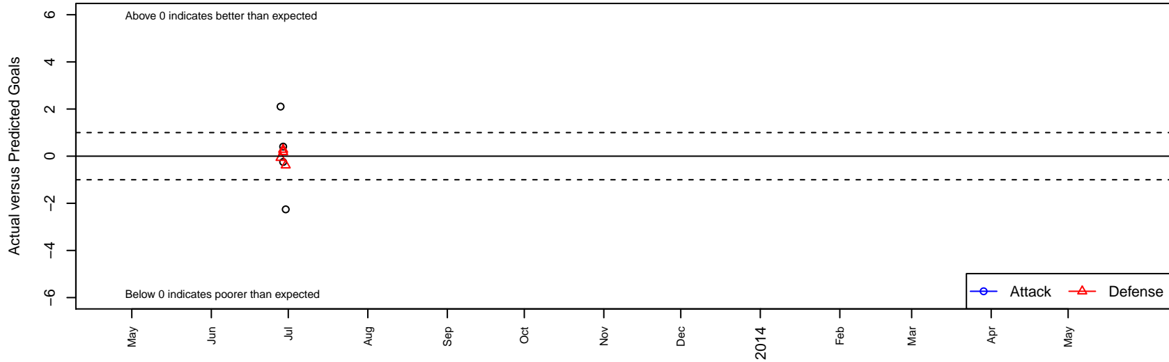
CYSA Timber Barons –Unk G01 Dots are actual minus expected GF (blue circles) and GA (red triangles). Blue line is smoothed change in attack strength. Red is smoothed change in defense strength.
